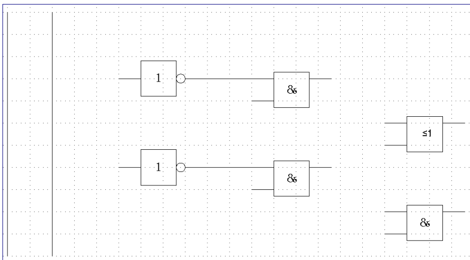
Figure 11: Drawing a half adder - Step 3
