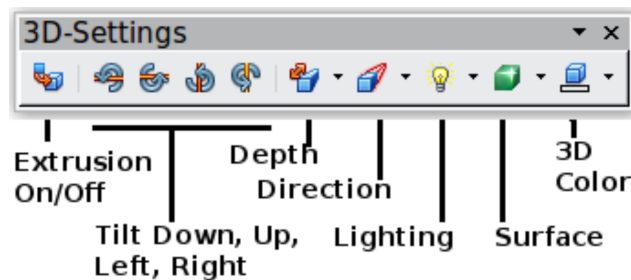
Figure 15: 3D-Settings toolbar
