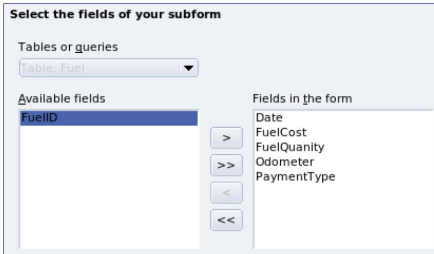
Figure 190: Selecting fields of a subform
