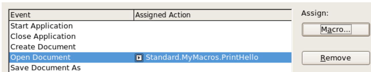
Figure 313: PrintHello is assigned to the Open Document event
