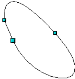
Figure 25: Closing an open curve
