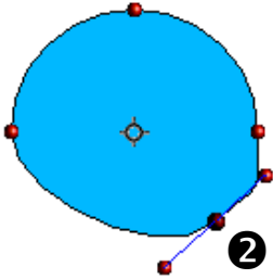
Figure 27: Moving a point on a curve
