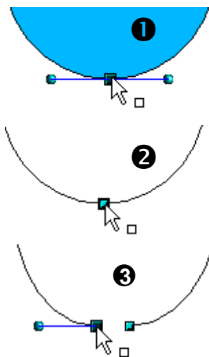
Figure 23: Cutting a curve
