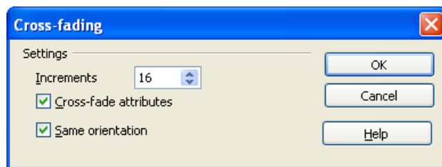
Figure 32: Cross-fading dialog
