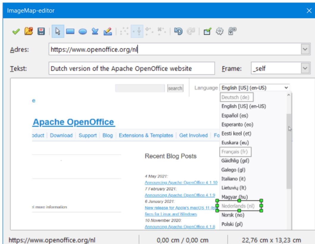
Figure 6: The dialog to create or edit an image map
